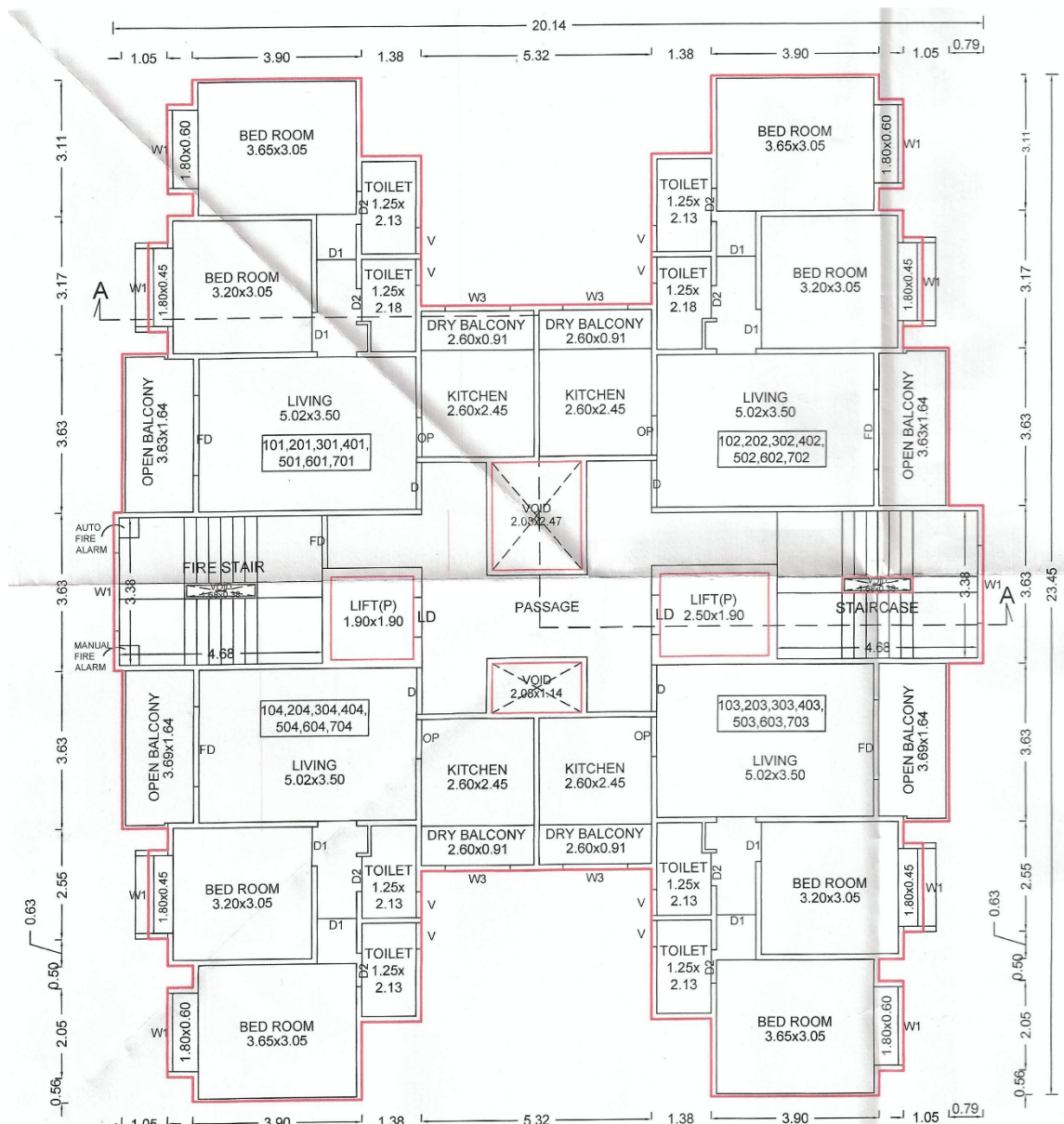
TYPICAL - 1, 2, 3, 4, 5, 6 & 7 FLOOR PLAN
