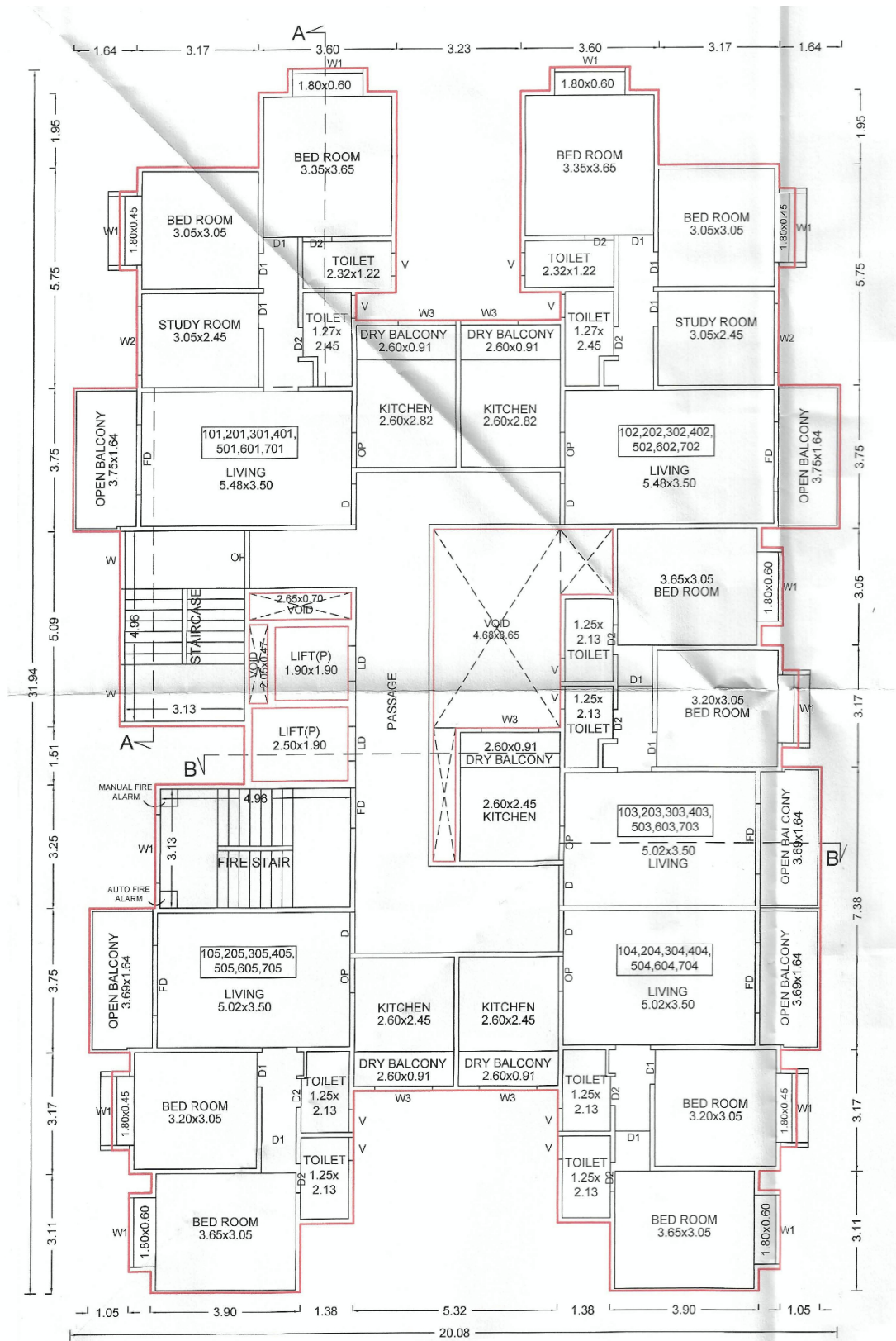
TYPICAL - 1, 2, 3, 4, 5,6 & 7 FLOOR PLAN
