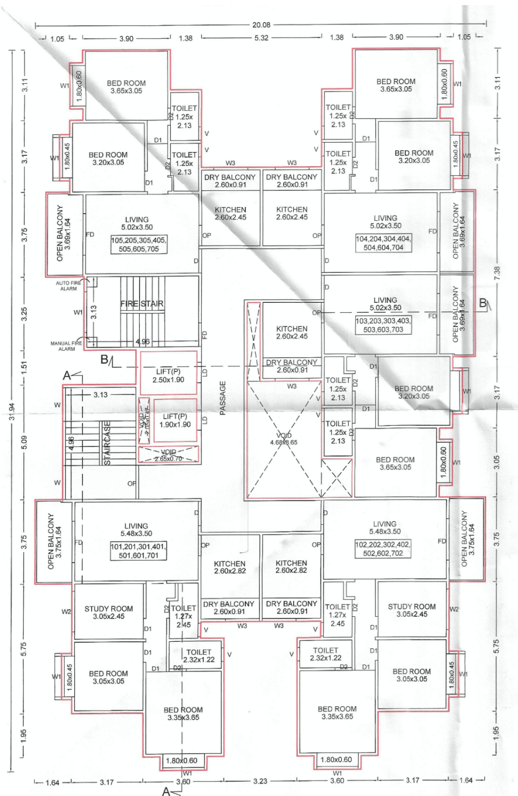
TYPICAL - 1, 2, 3, 4, 5, 6 & 7 FLOOR PLAN BUILDING - D FLAT NO. _____
