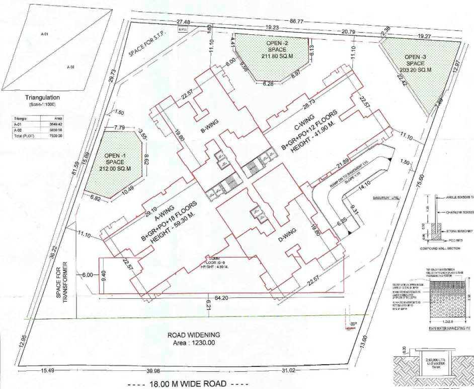
LAYOUT PLAN (SCALE: 1:250)
